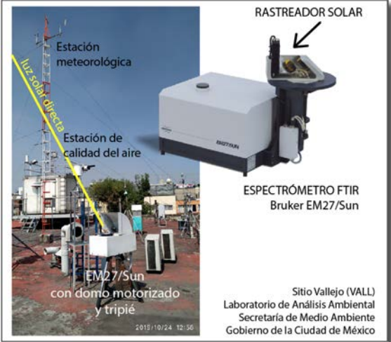
Percepción Remota Columna CO 2 (EM27/Sun)
